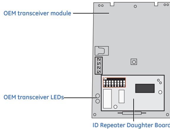
Figure 3. ID Repeater Daughter Board mounted on the OEM transceiver
