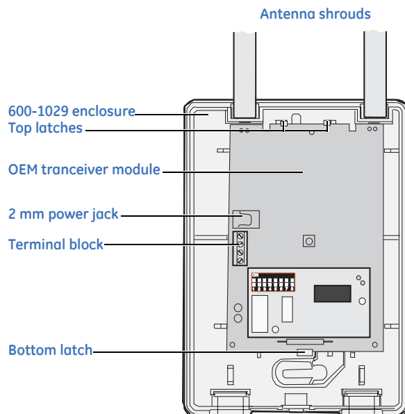
Figure 4. OEM transceiver module mounted in the 600-1029 enclosure
